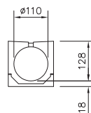
Canal SlimLine 50cm Canal SlimLine 50cm
